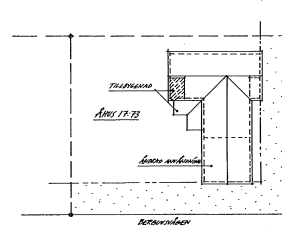
SITUATIONSPLAN 1:200
